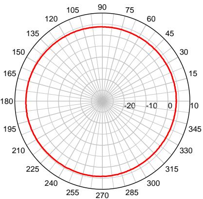
SMW 1900 MHz – Azimuth Plot
